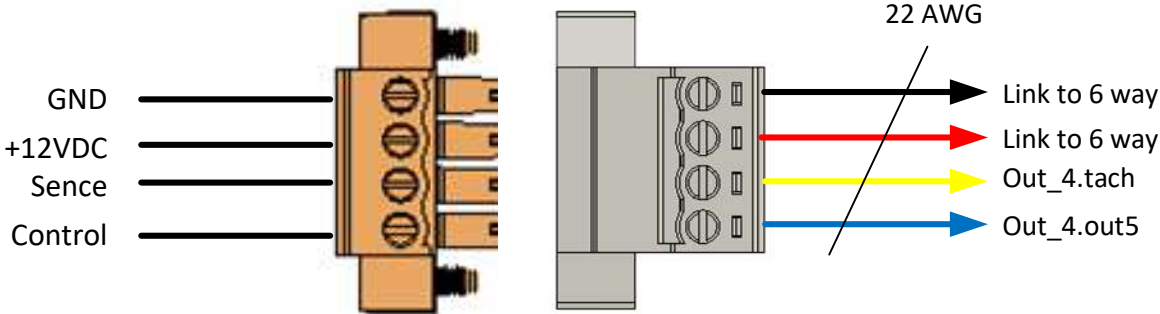
Sleeve cables
